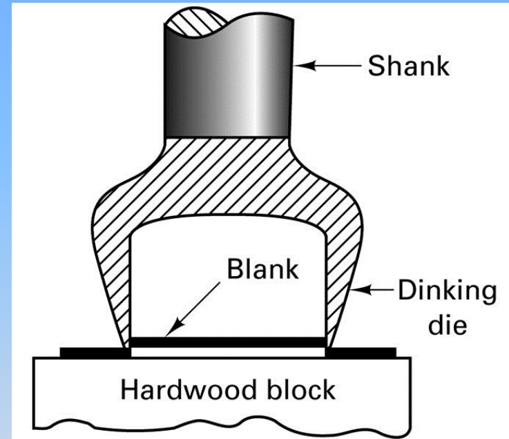
Figure 17-10 The dinking process.
