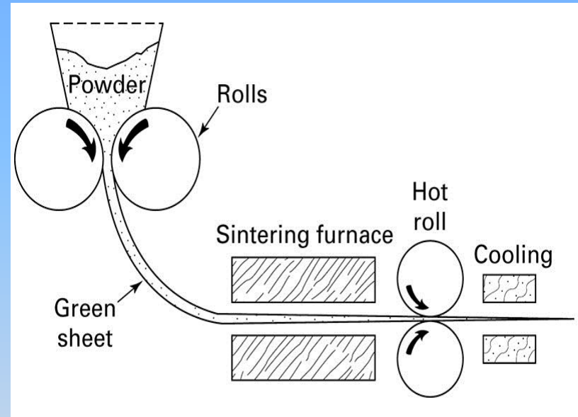
Figure 18-11 One method of producing continuous sheet products from powdered feedstock.
