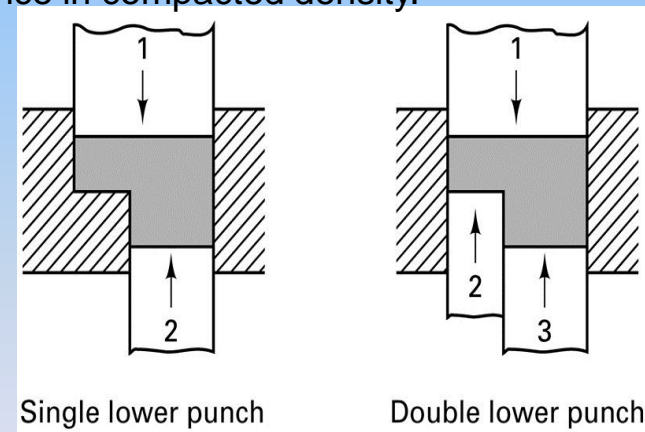
Figure 18-9 Two methods of compacting a double-thickness part to near-uniform density. Both involve the controlled movement of two or more punches.
