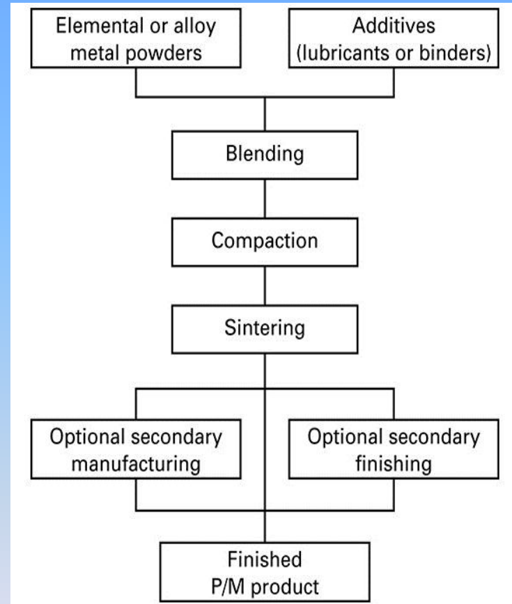
Figure 18-1 Simplified flow chart of the basic powder metallurgy process.
