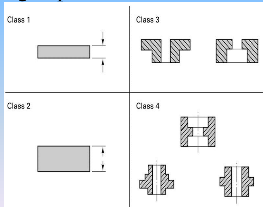
Figure 18-10 Sample geometries of the four basic classes of press-and-sinter powder metallurgy parts. Note the increased pressing complexity that would be required as class increases.
