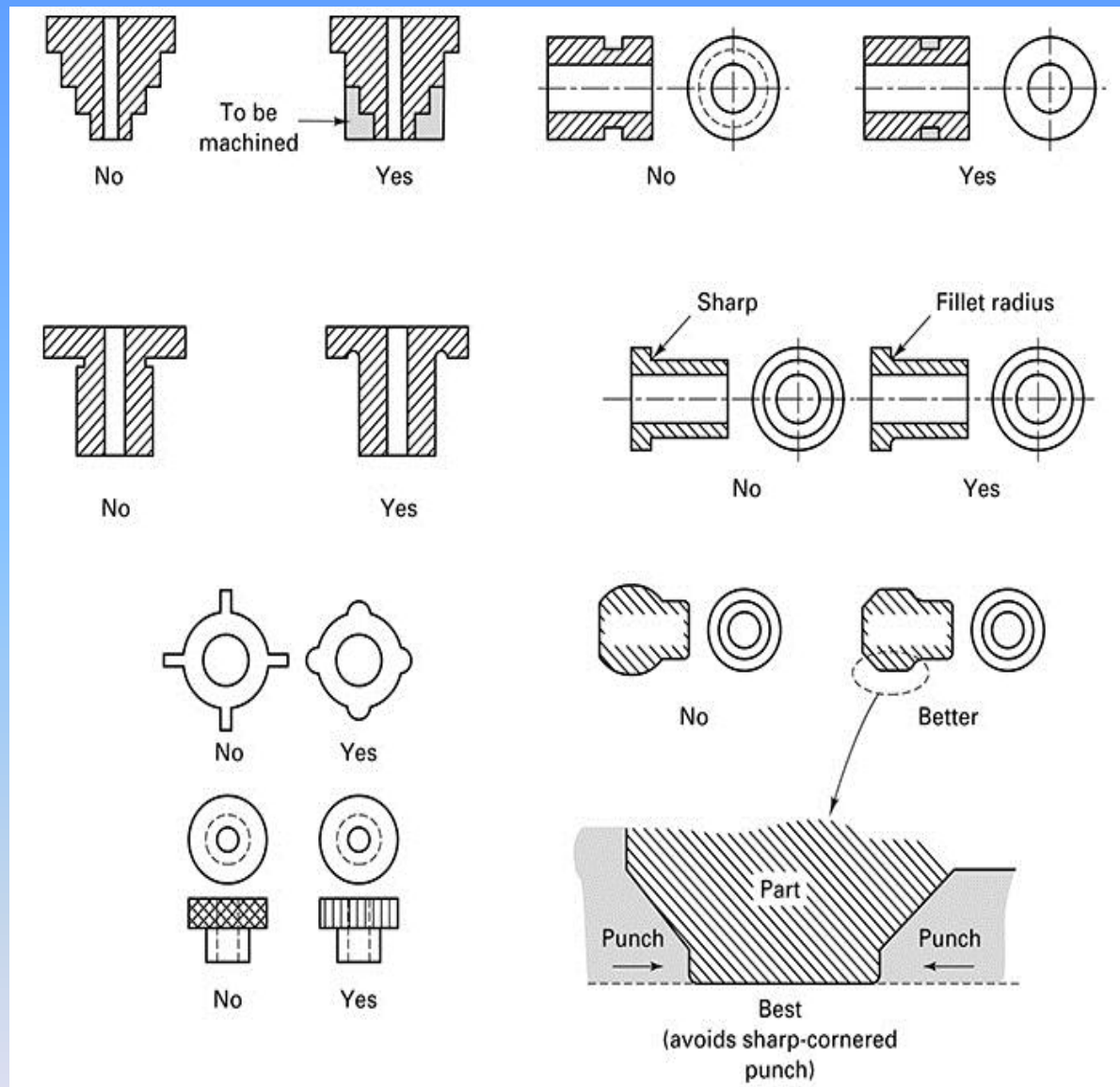
Figure 18-17 Examples of poor and good design features for powder metallurgy products. Recommendations are based on ease of pressing, design of tooling, uniformity of properties, and ultimate performance.
