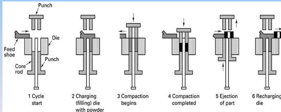
Figure 18-4 Typical compaction sequence for a single-level part, showing the functions of the feed shoe, die core rod, and upper and lower punches. Loose powder is shaded; compacted powder is solid black.
