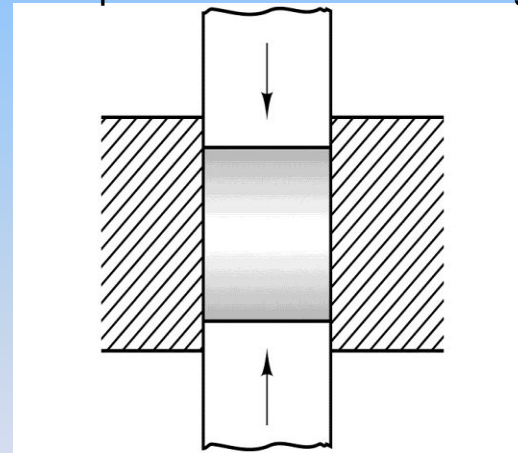
Figure 18-6 Density distribution obtained with a double-acting press and two moving punches. Note the increased uniformity compared to Figure 18-5. Thicker parts can be effectively compacted.
