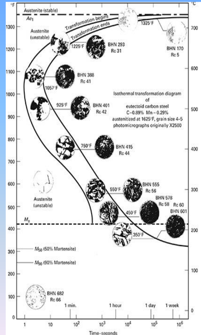
Figure 5-7 Isothermal transformation diagram (T-T-T diagram) for eutectoid composition steel. Structures resulting from transformation at various temperatures are shown as insets. (Courtesy of United States Steel Corp., Pittsburgh, PA.)
